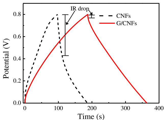
Fig. 6. Galvanostatic charge–discharge curves of CNF (black) and G/CNF (red) samples at a constant current density of 500 \text{mA g}^{-1} . (For interpretation of the references to color in this figure legend, the reader is referred to the web version of this article.)
