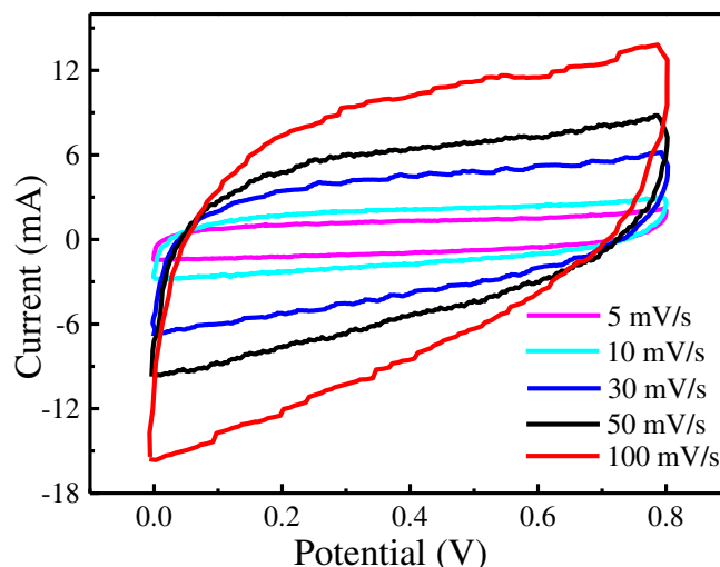
Fig. 5. Cyclic voltammograms of G/CNF samples at a varying scan rate in the range of 5–100 \text{mV s}^{-1} .
