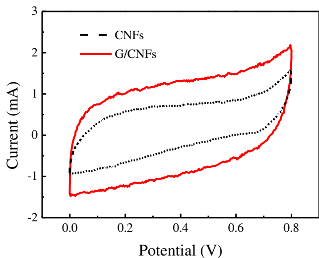
Fig. 4. Cyclic voltammograms of CNF (black) and G/CNF (red) samples at a scan rate of 5 \text{mV s}^{-1} in a 6 M KOH solution. (For interpretation of the references to color in this figure legend, the reader is referred to the web version of this article.)
