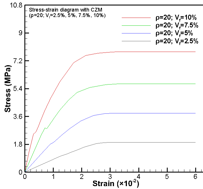
Figure 13. Effective stress-strain diagrams of the PNC (stack nanoparticle configuration) with CZM at the nanoparticle volume fraction of V_f = 2.5\% , 5%, 7.5%, and 10%, respectively ( q = 20 ).
