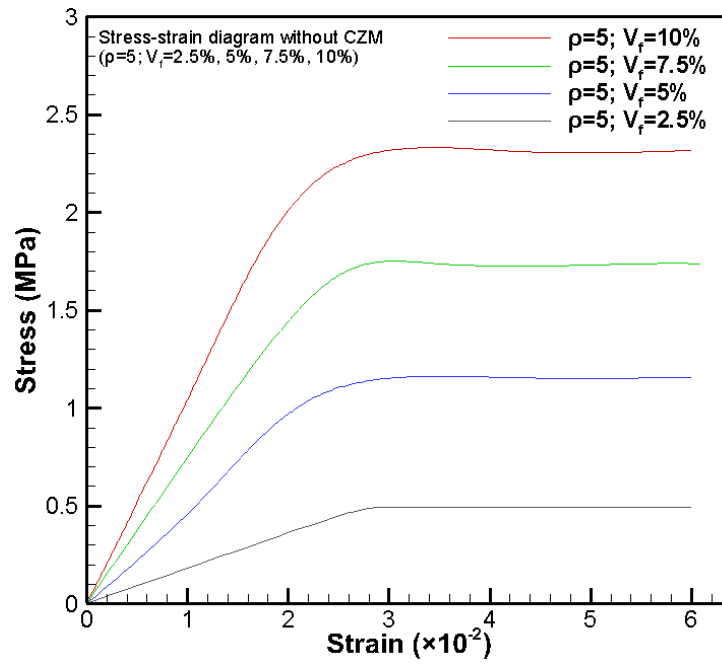
Figure 15. Effective stress-strain diagrams of the PNC (stack nanoparticle configuration) without CZM at the nanoparticle volume fraction of V_f = 2.5\% , 5%, 7.5%, and 10%, respectively ( \rho = 5 ).
