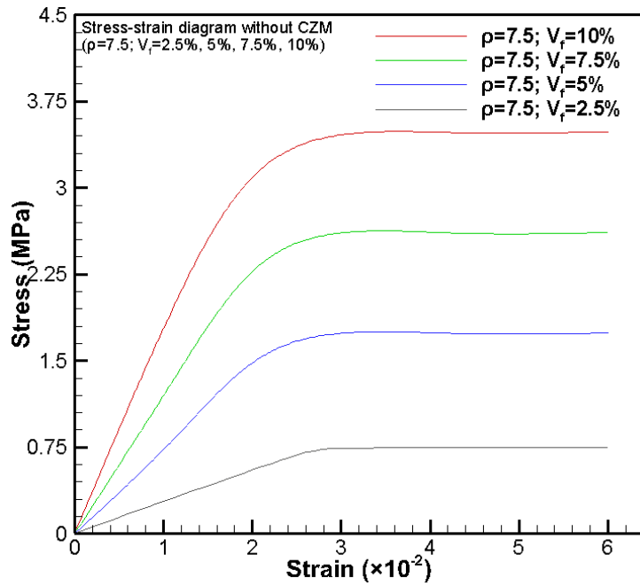
Figure 16. Effective stress-strain diagrams of the PNC (stack nanoparticle configuration) without CZM at the nanoparticle volume fraction of V_f = 2.5\% , 5%, 7.5%, and 10%, respectively ( \rho = 7.5 ).
