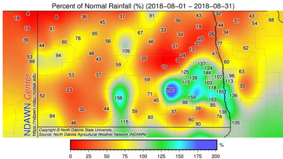
Figure 1. August 2018 precipitation percent of normal for North Dakota. (NDAWN Center, NDSU)
