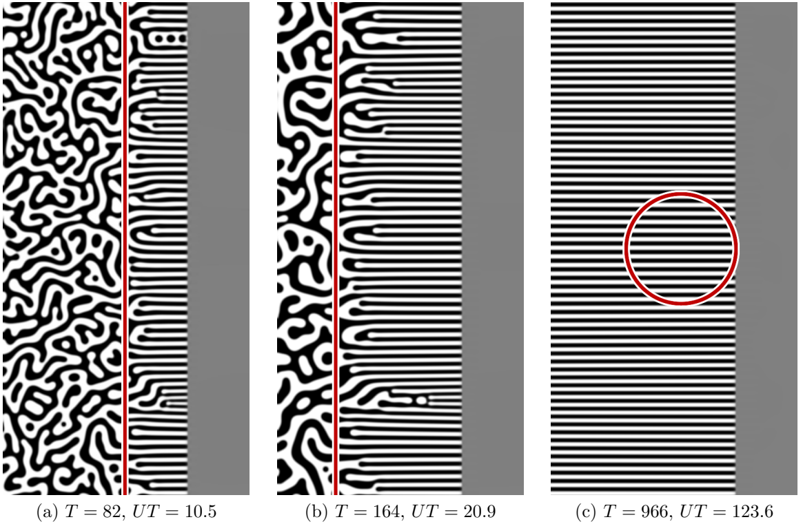
Figure 19. (Color online) Stripe formation in the wake of a phase separation front as seen in an LBM simulation at U = 0.128 and symmetric mixed material concentration \Phi = 0 . The starting location of the front is marked as a vertical stripe. The rightmost image is the final structure observed after the front has moved far into the material. A sample of the final morphology, noted by the circled region, will be compared to samples from other simulations performed with different parameter values.
