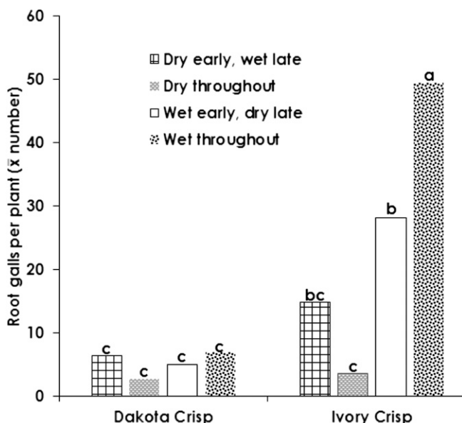
Fig. 1. Mean number of Spongospora subterranea f. sp. subterranea galls on roots across soil moisture regimes in Dakota Crisp and Ivory Crisp. Data represent the interaction between moisture regime and cultivar on root gall formation based on data combined after two trials. Means with the same letter are not significantly different based on Fisher's protected least significance difference ( P < 0.05 ).
