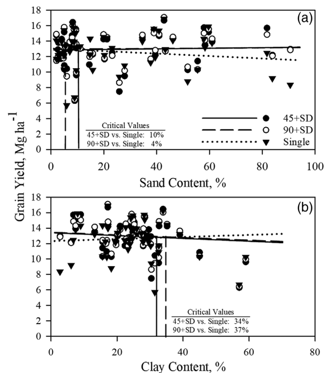
FIGURE 1 Examples of the two interpretations of critical values using the relationships between grain yield and sand (a) and clay (b) content (0–30 cm) for a single-N vs. two split-N applications (45 kg ha -1 at planting and remaining at ~V9 [45+SD] or 90 kg ha -1 at planting and remainder at ~V9 [90+SD]) at a total of 180 kg ha -1 ( P \leq .05 ). a) Critical values for sand contents represents the point where smaller values were associated with greater grain yield with single-N applications and larger values were associated with greater grain yield with split-N applications. b) Critical values for clay content represent the point where smaller values were associated with greater grain yield with split-N applications and larger values were associated with greater grain yield with a single-N application
