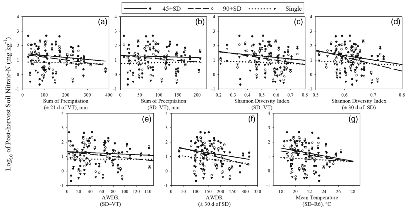
FIGURE 4 Post-harvest soil \text{NO}_3\text{-N} (0–90 cm) as a function of the sum of precipitation (a, b), Shannon Diversity Index (c, d), Abundant and Well-Distributed Rainfall (AWDR) (e, f) and mean temperature (g) from sidedress (SD) to VT or R6 or 21–30 d before and after SD or VT of a single- and two split-N applications ( 45 \text{ kg ha}^{-1} at planting and remainder at \sim\text{V9} [45+SD] or 90 \text{ kg ha}^{-1} at planting and remainder at \sim\text{V9} [90+SD]) across two N rates ( 180 and 270 \text{ kg ha}^{-1} ) and 49 site-years. Only soil or weather variables that had a significant interaction with N application timing are shown ( P \leq .05 ). R-square values were \leq 0.06
