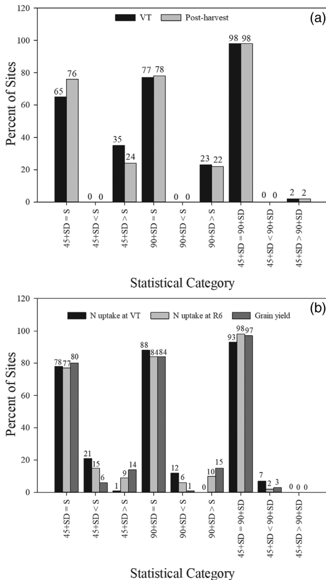
FIGURE 2 Statistical categories comparing the percent of sites with similarities and differences in a) soil NO 3 -N concentration at VT (0–60 cm) and post-harvest (0–90 cm), and b) plant N uptake at VT and R6 and grain yield among three N application timings (single-N application at planting [S] and two split applications with 45 [45+SD] or 90 kg ha -1 [90+SD] at planting and the remainder applied at ~V9) across 45 and 49 site-years for VT and post-harvest soil NO 3 -N, respectively. Comparisons for soil NO 3 -N at VT were made at the 180 kg N ha -1 rate only; post-harvest soil NO 3 -N included both 180 and 270 kg N ha -1 rates
