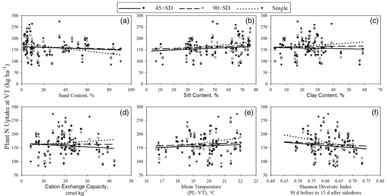
FIGURE 5 Plant N uptake at VT as a function of soil (a, b, c, d) and weather conditions (e, f) from planting (PL) to VT (e) and 30 d before and 15 d after sidedress N application of a single- and two split-N applications (45 kg ha -1 at planting and remaining at ~V9 [45+SD] or 90 kg ha -1 at planting and remainder at ~V9 [90+SD]) across two N rates (180 and 270 kg ha -1 ) and 47 site-years. Only soil or weather variables that had a significant interaction with N application timing are shown ( P \leq .05 ). R-square values were \leq 0.14
