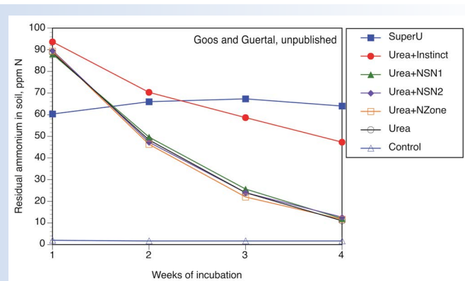
Figure 15. Ammonium-N remaining in the soil after application of Urea and amendments through time. NSN1 and NSN2 are formulations of Nutrisphere-N. Super U contains DCD.
